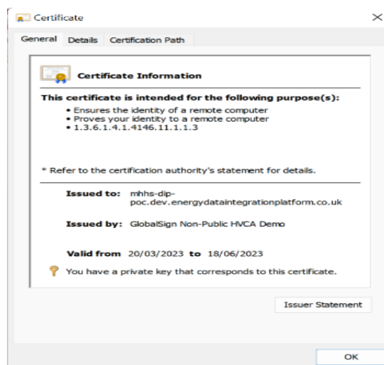
Figure 1 - Digital Certificate.
