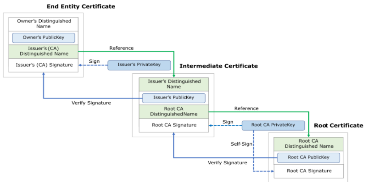
Figure 4 - Certificate Chain.
