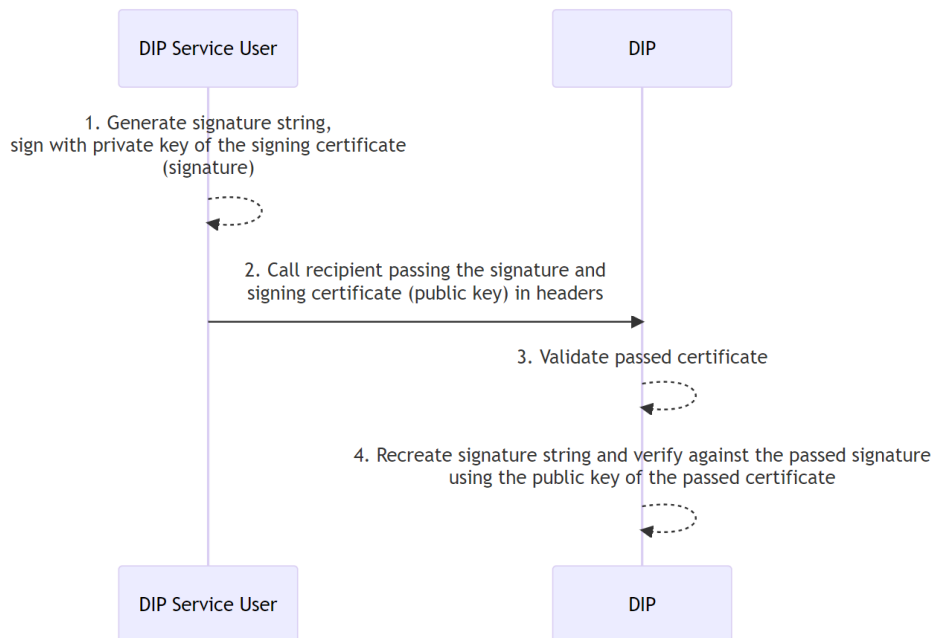
Figure 14 - Message signing ingress flow
